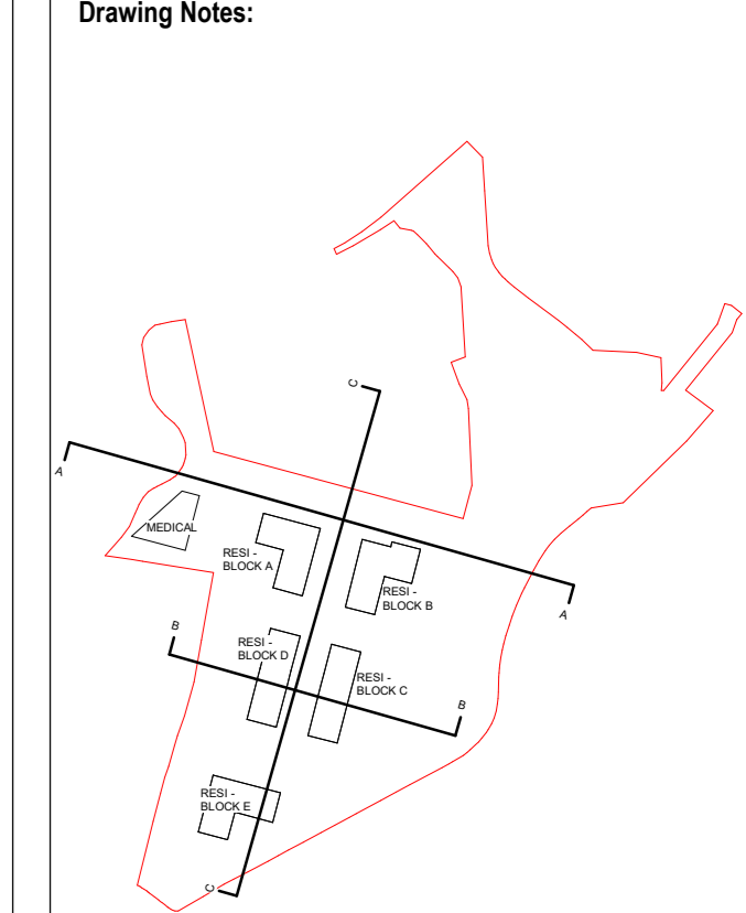
Site Sections - Keyplan 1:5000
