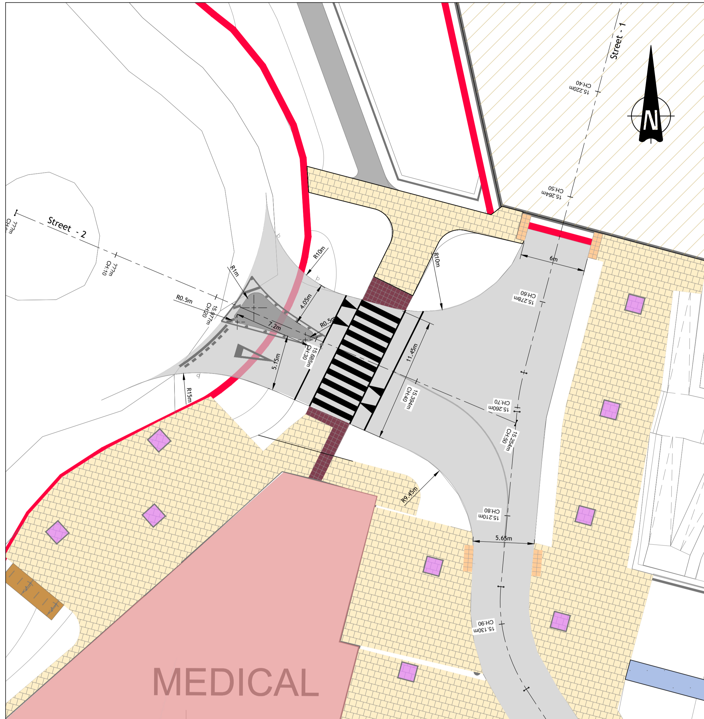
PROPOSED ROUNDABOUT MODIFICATIONS LAYOUT SCALE 1:200
