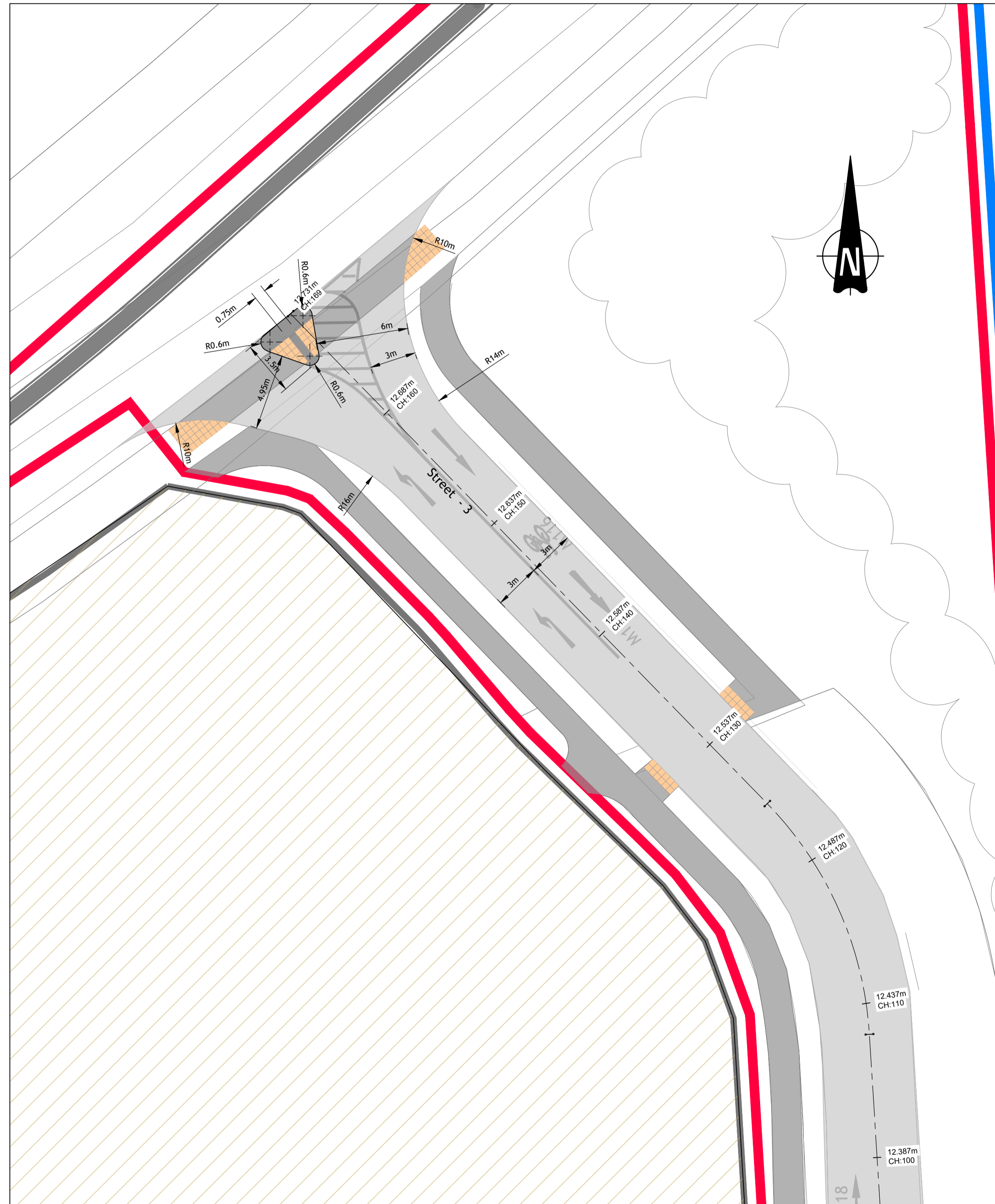
PROPOSED DUBLIN ROAD JUNCTION LAYOUT SCALE 1:200
