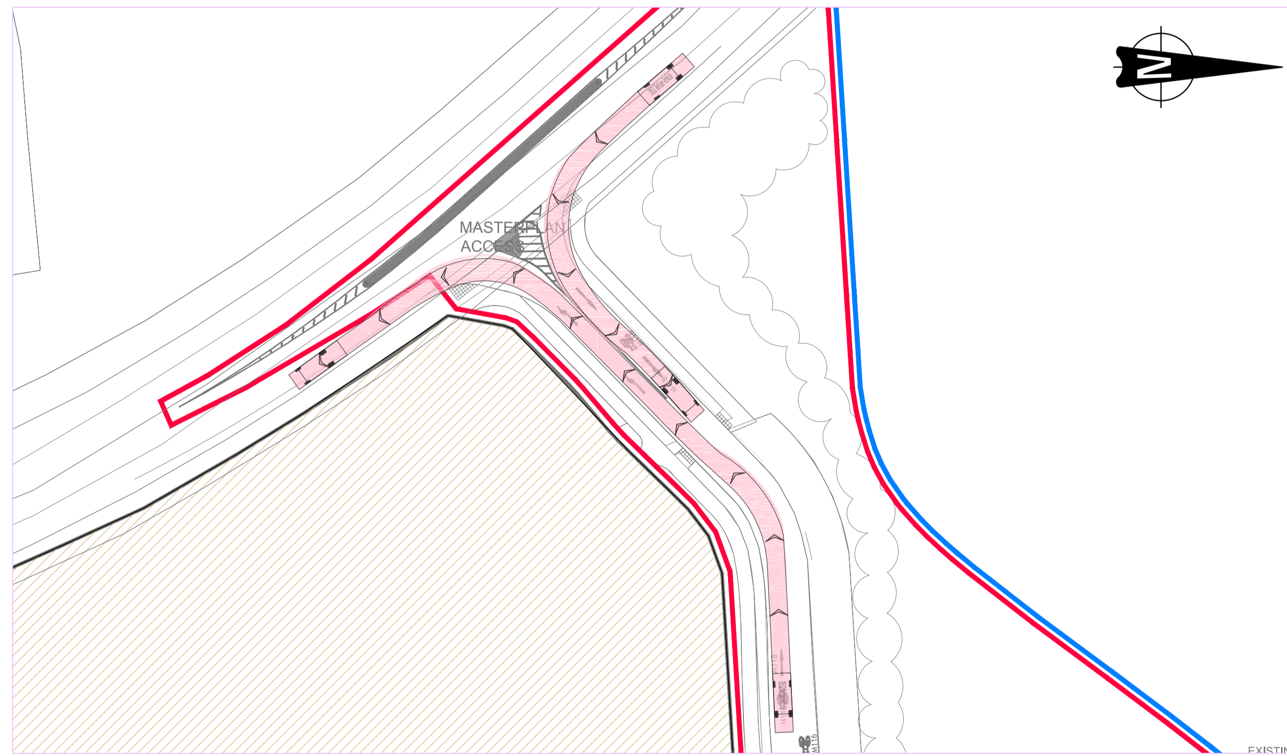
DETAIL 3 REFUSE TRUCK - ENTERING AND EXITING AT PROPOSED DUBLIN ROAD LAYOUT Scale 1:250
