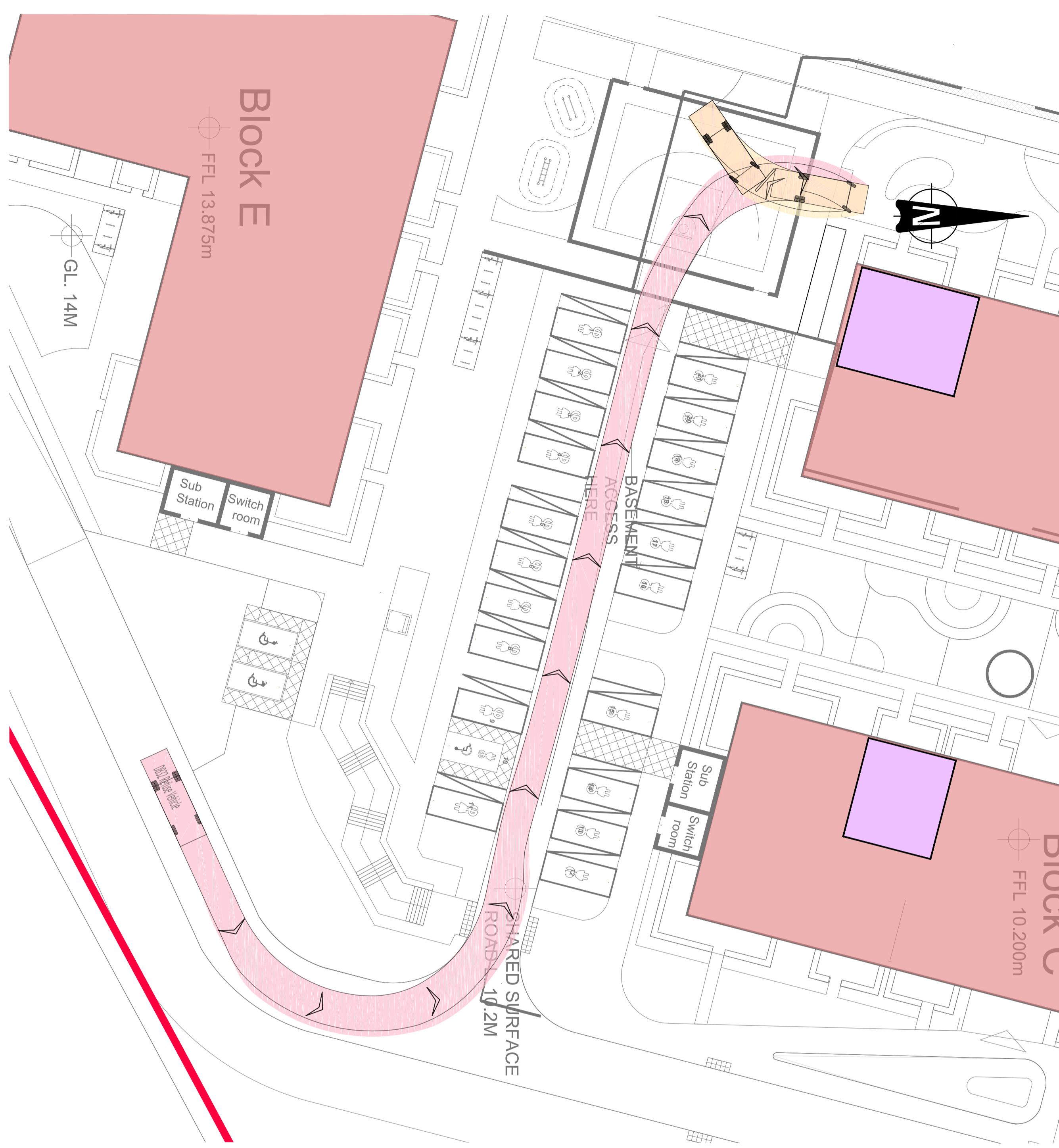
DETAIL 2 - REFUSE TRUCK - ENTERING AND EXITING THE BASEMENT BLOCK D SCALE 1:250
