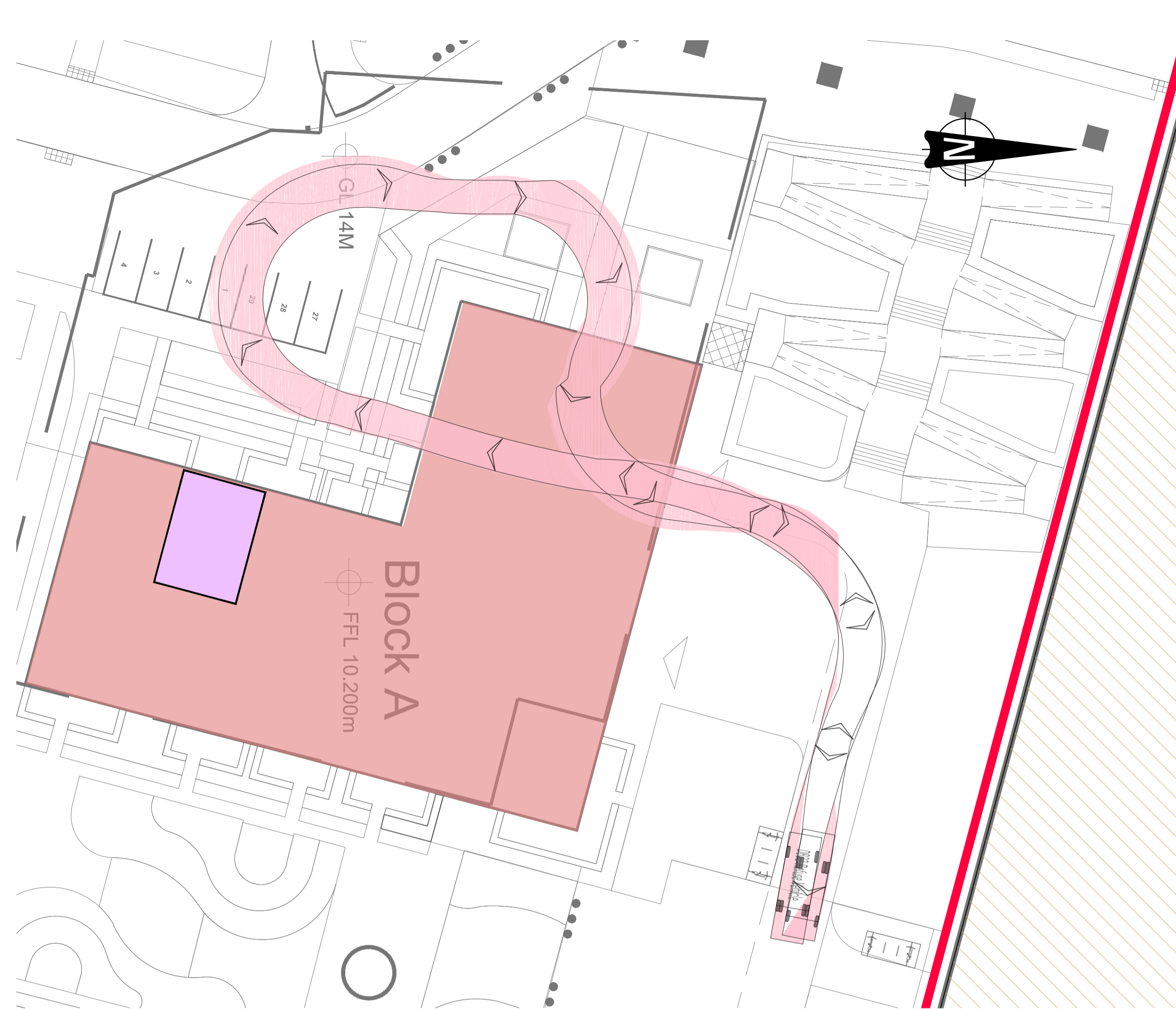
DETAIL 1 - REFUSE TRUCK - ENTERING & EXITING BASEMENT BLOCK A SCALE 1:250
