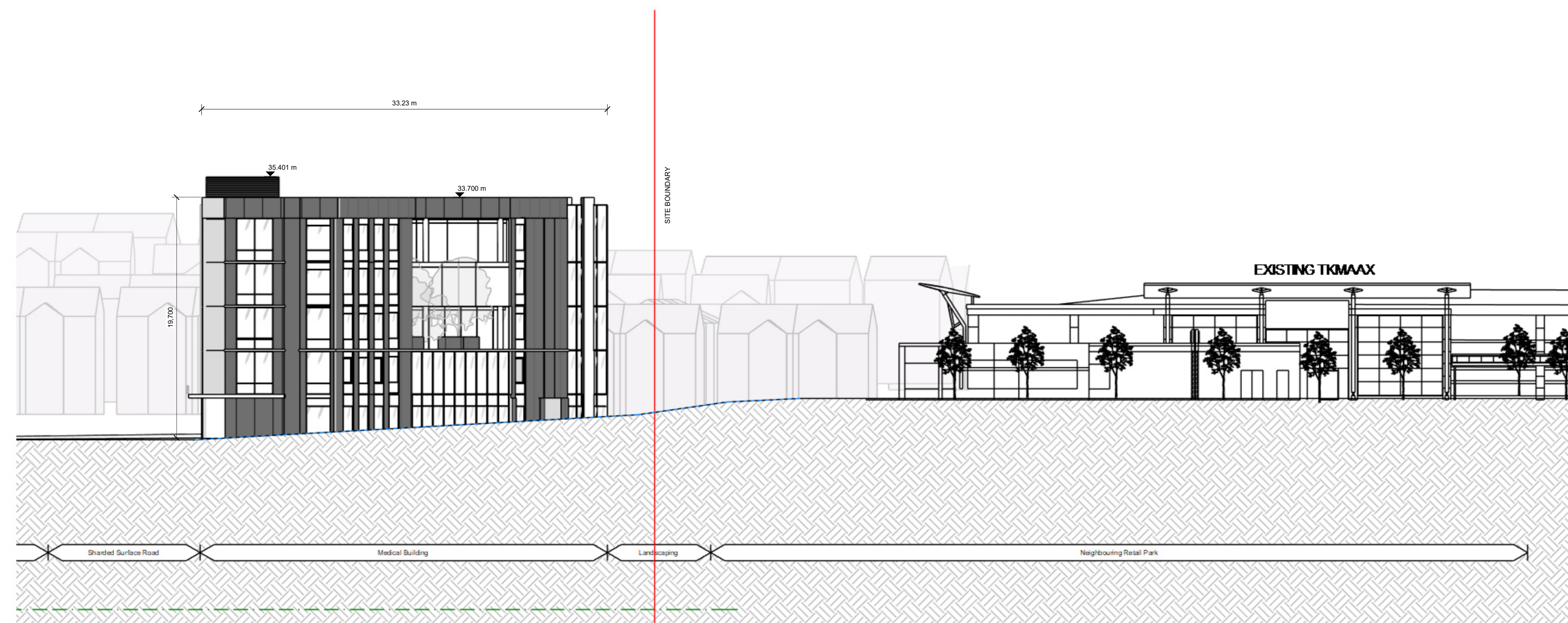
Sectional Elevation A-A - Zone 02 1:200
