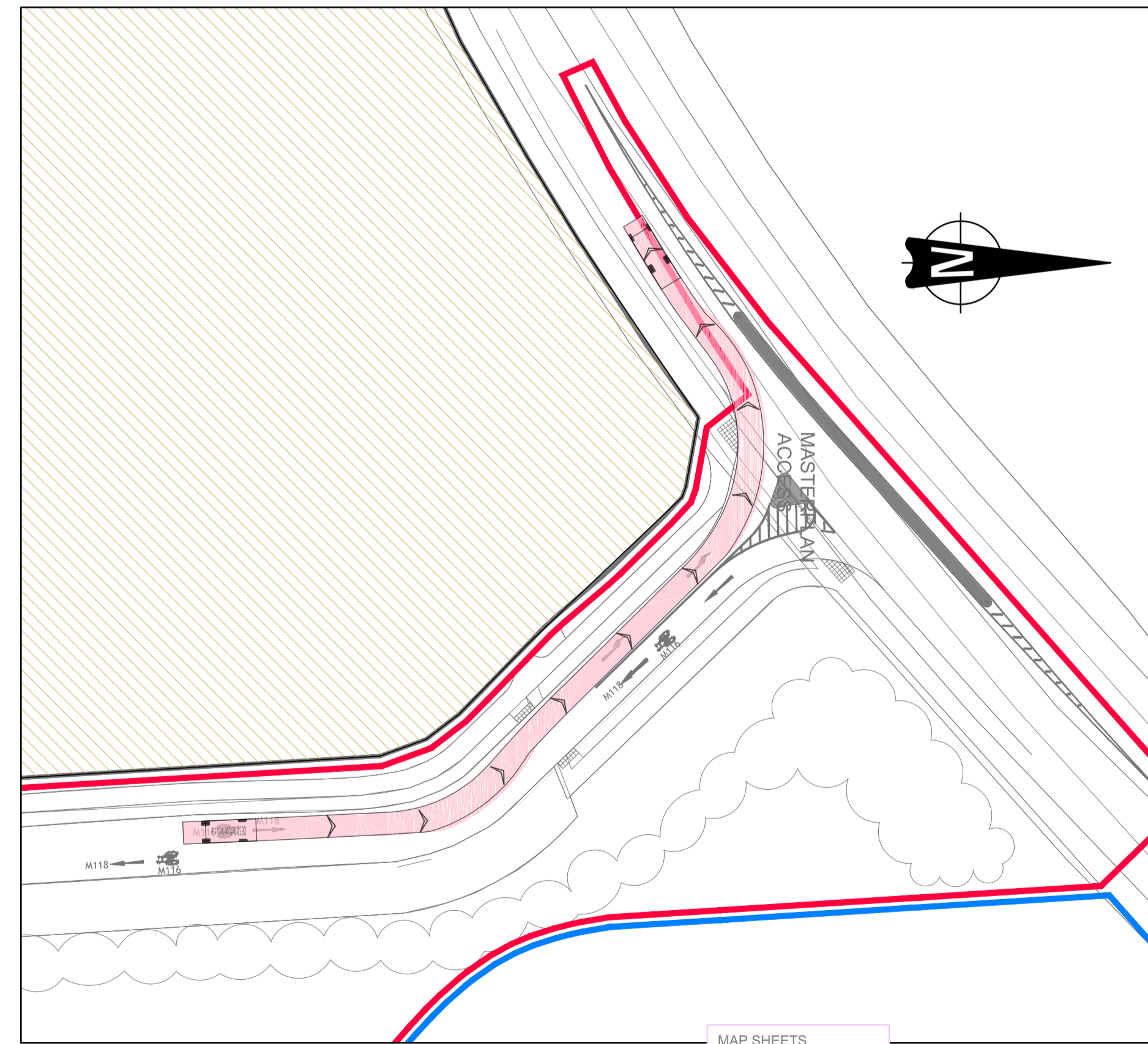
DETAIL 2 - REFUSE TRUCK - ENTERING & EXITING THE SITE VIA DUBLIN ROAD SCALE 1:500
