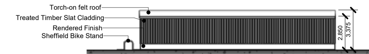
Bike Store Elevation East 1 : 200
