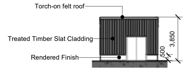
Substation - East Elevation 1 : 200
