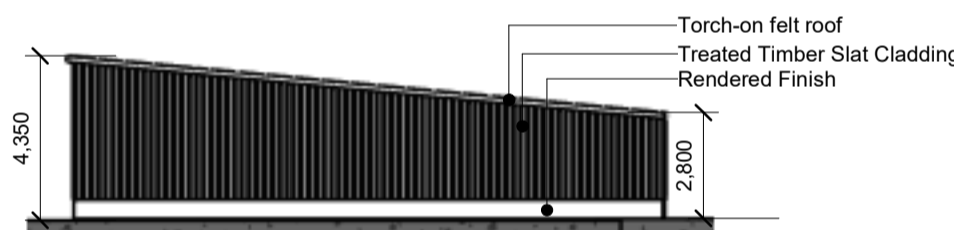
Pump Station - South Elevation 1 : 200
