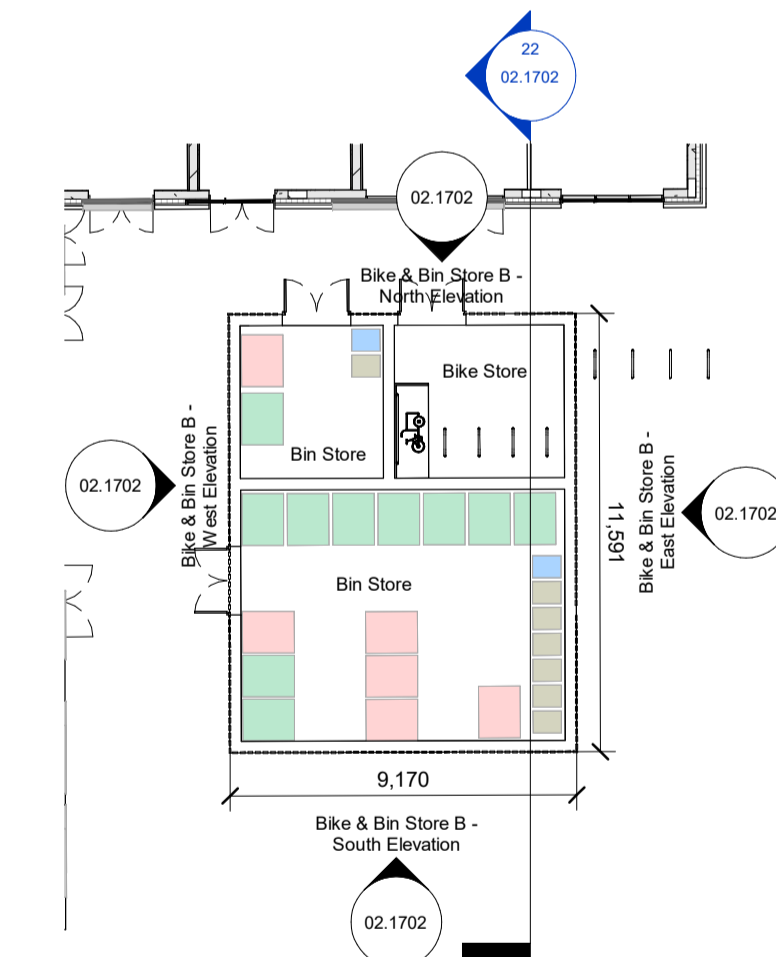
L00 - Site Plan - Bike & Bin Store 1 : 200
