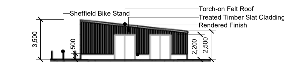
Bike & Bin Store B - North Elevation 1 : 200
