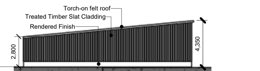
Pump Station - North Elevation 1 : 200
