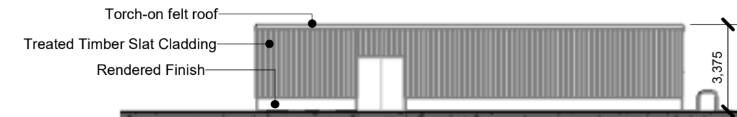
Bike Store Elevation West 1 : 200
