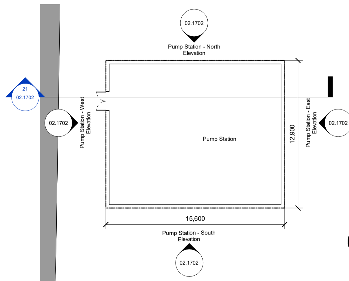
L00 - Site Plan - Pump Station 1 : 200
