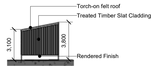
Substation - South Elevation 1 : 200
