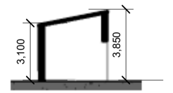
Substation - Section 1 : 200
