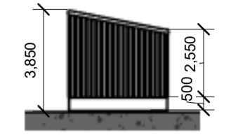
Substation - North Elevation 1 : 200
