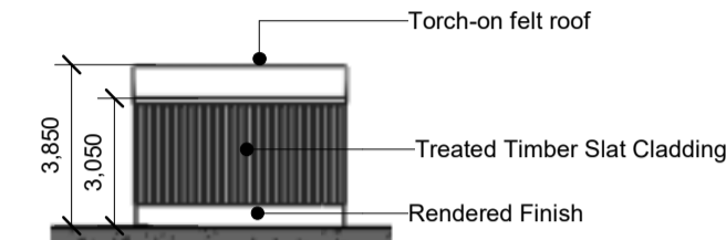
Substation - West Elevation 1 : 200
