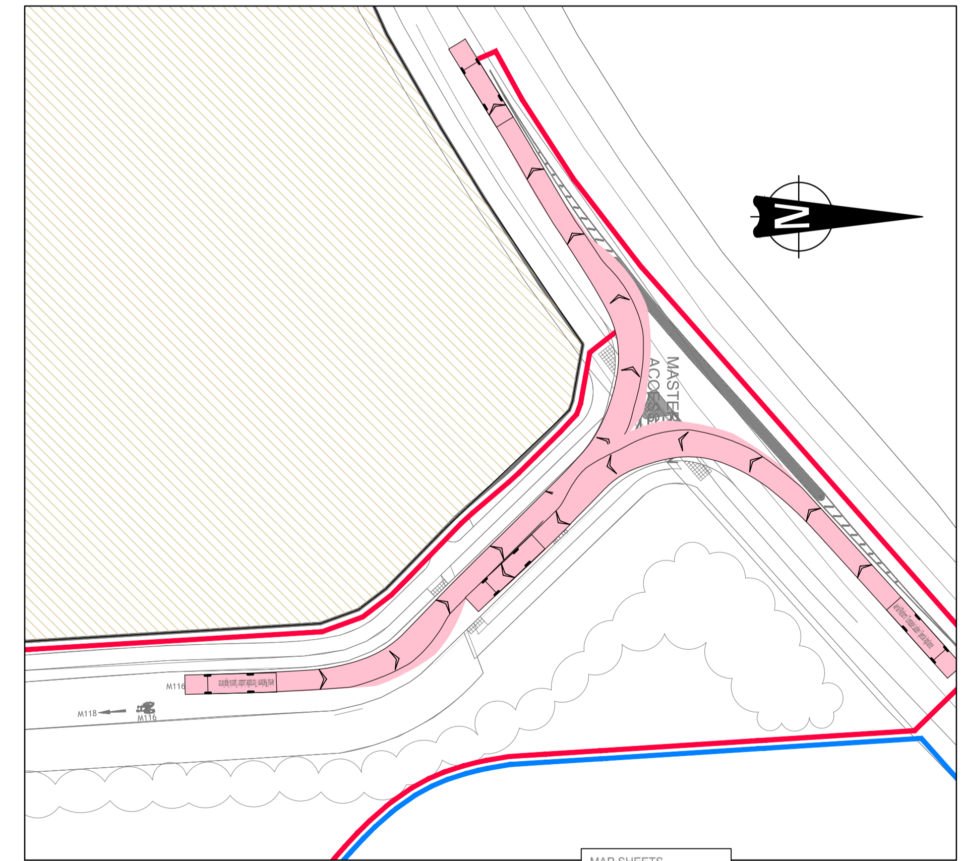
DETAIL 2 - FIRE TENDER - ENTERING & EXITING THE SITE VIA DUBLIN ROAD SCALE 1:500
